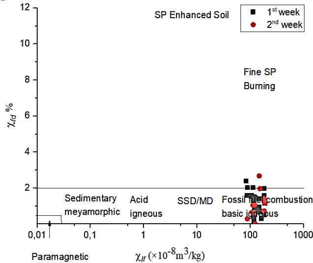
Fig 6. Relationship between low-frequency susceptibility ( \chi_{LF} ) ( 10^{-8} \text{ m}^3/\text{kg} ) and frequency-dependent susceptibility ( \chi_{FD}\% )
