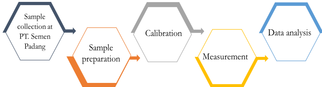
Fig 3. Flowchart of magnetic susceptibility analysis of Raw Mix I at PT Semen X.
